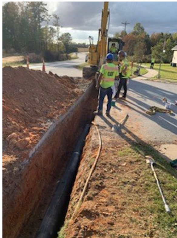
Photo 4: Line install
